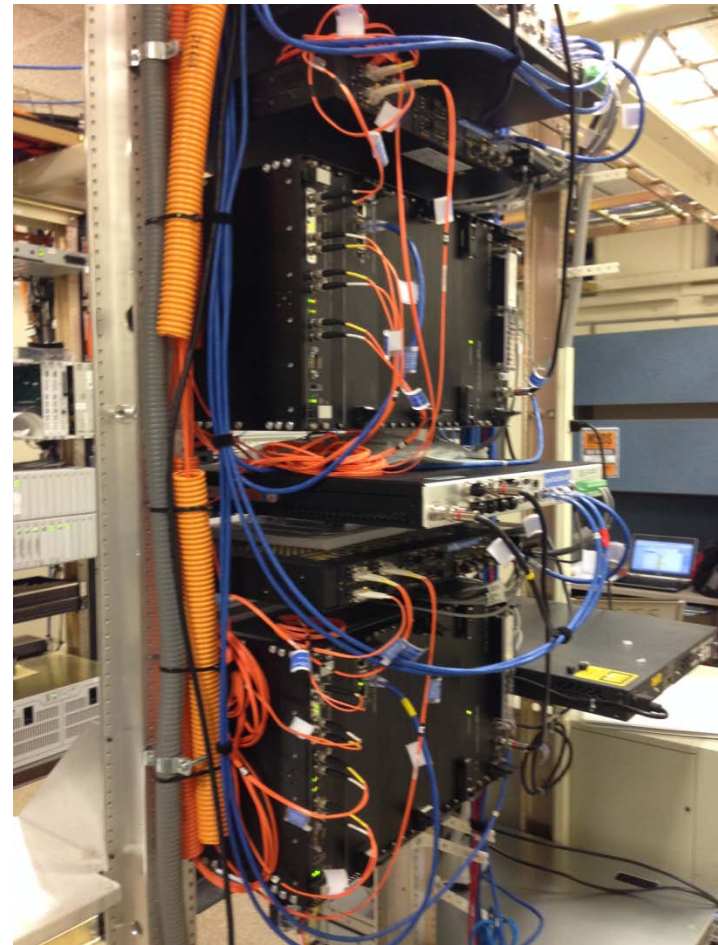
Typical PDC field installation
